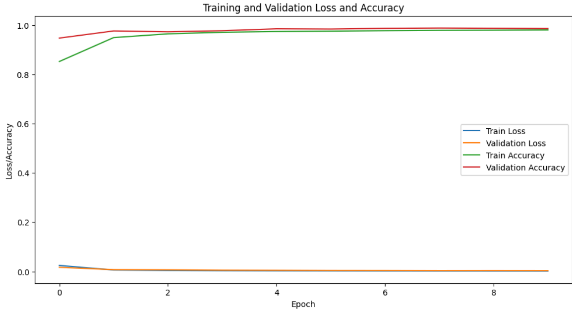
Fig. 3.5: Training and Validation Loss and Accuracy Before Hyperparameter Tuning
