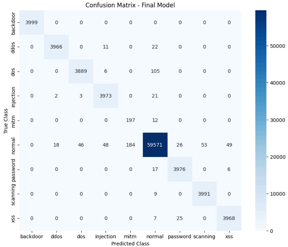
Fig. 3.4: Confusion Matrix After Hyperparameter Tuning
